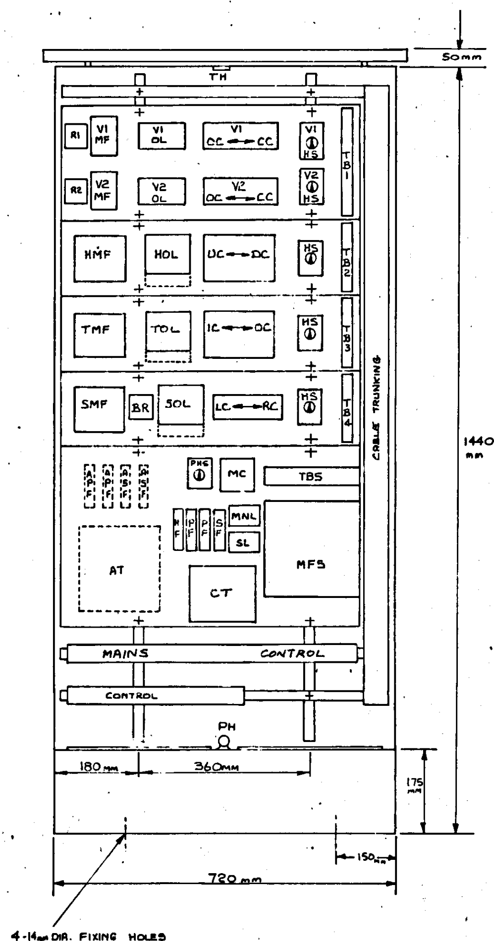
LAYOUT FOR BARGE LOADING/SHIPPING SPOUTS-PANELS MCC6A-6F — SEAFORTH GRAIN TERMINAL
